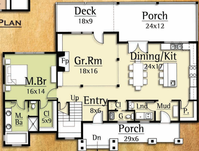
MAIN LEVEL PLAN
